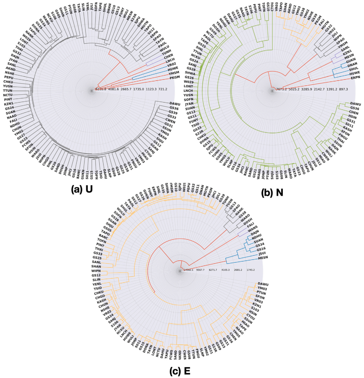
Fig. 5. Resulting dendrogram for the HAC method as a polar chart for the (a) vertical, (b) north, and (c) east component GNSS residuals of Taiwan. The figure is auto-generated using the dtwhaustering package.
